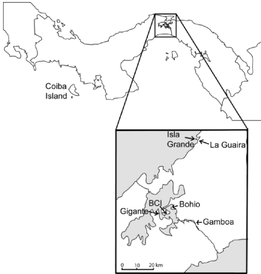
FIG. 1.—Sampling sites.
