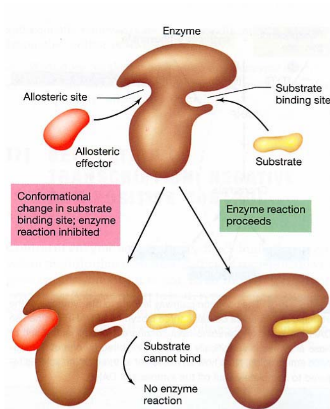
Figure 8.3 Mechanism of enzyme inhibition by an allosteric effector. When the effector combines with the allosteric site, the conformation of the enzyme is altered so that the substrate can no longer bind.
