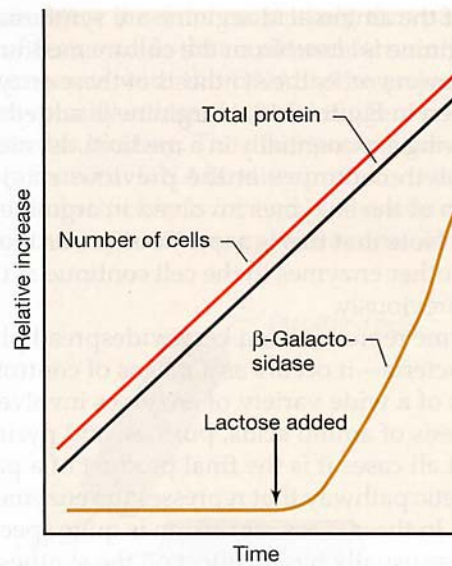
Figure 8.11 Induction of the enzyme \beta -galactosidase on the addition of lactose to the medium. Note that the rate of total protein synthesis remains unchanged.
