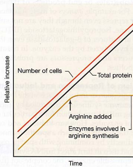
Figure 8.10 Repression of enzymes involved in arginine synthesis by addition of arginine to the medium. Note that the rate of total protein synthesis remains unchanged.
