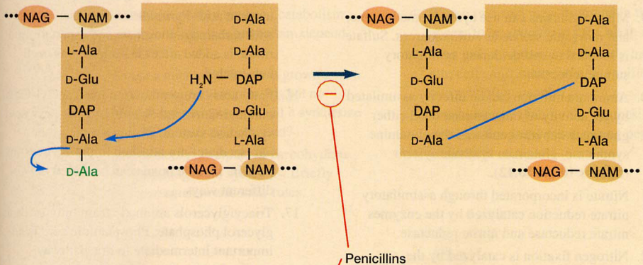
Figure 10.29 Transpeptidation. The transpeptidation reactions in the formation of the peptidoglycans of Escherichia coli and Staphylococcus aureus .
